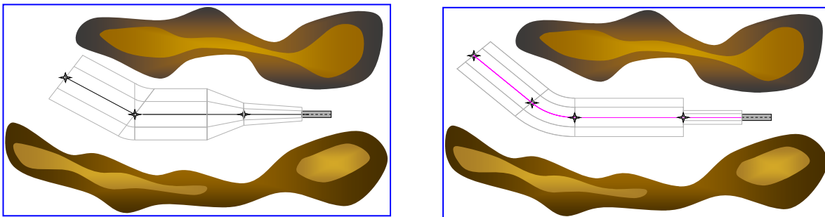
Figure 3-6: Examples of RNP APCH (left) and RNP AR APCH (right) procedure design
