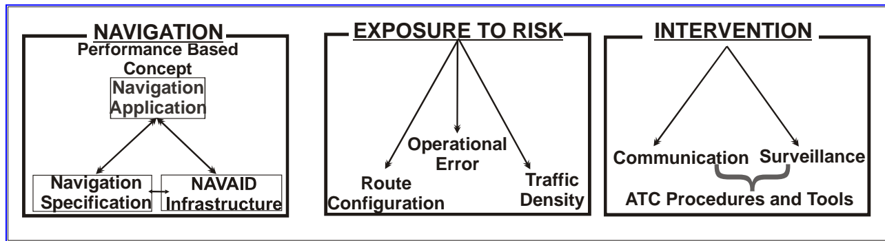
Figure 3-2: Generic model used to determine separation and ATS Route spacing
